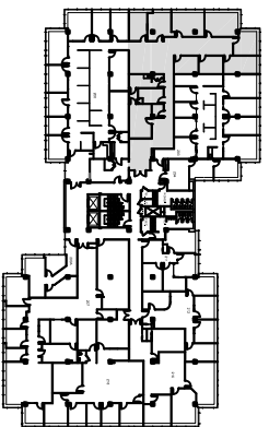
SECOND FLOOR KEY PLAN
